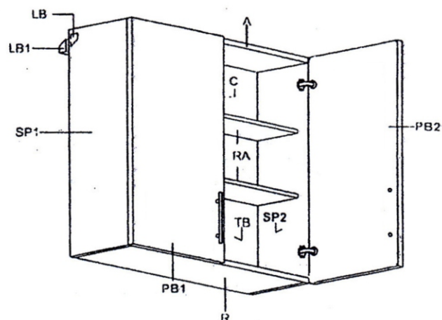
FINAL ASSEMBLING
